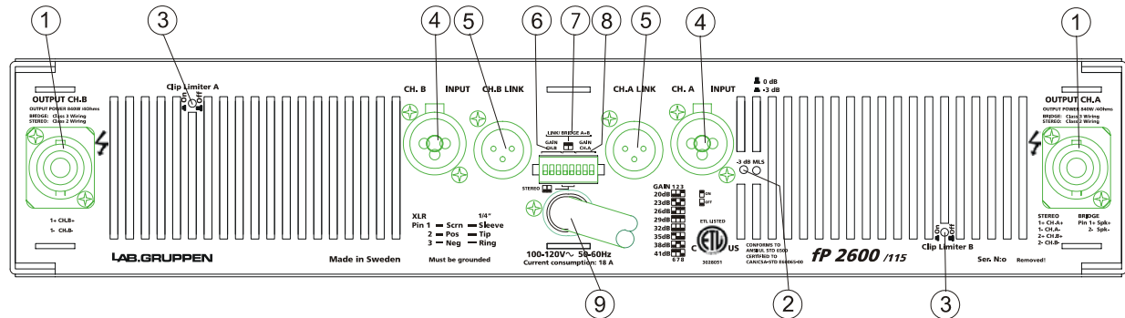
Figure 2: Rear panel
