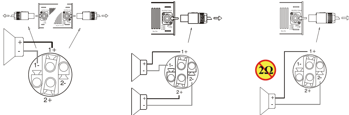
Channel A and B into one Speakon (Stereo and Bi-amp)
