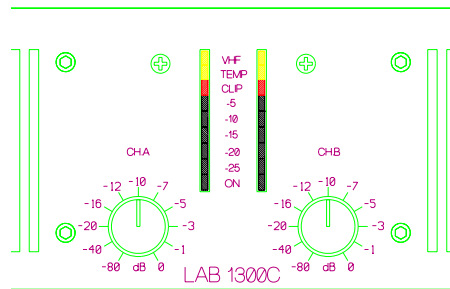
Figure 12. Front indicators
