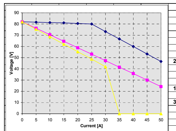
Figure 13. Current-voltage characteristic of different power supply topologies.
