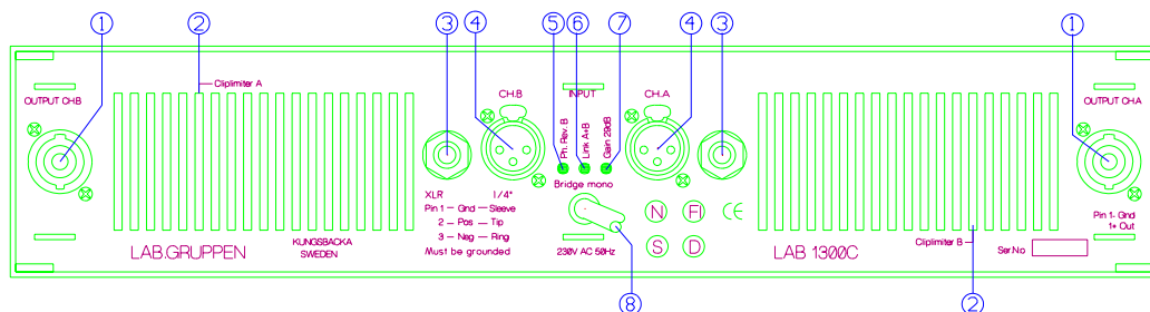
Figure 2. Rear panel
