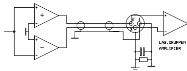
Figure 6. Balanced line
