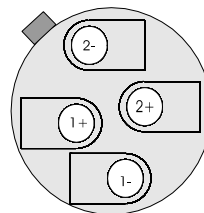
Figure 9. Speakon connector
