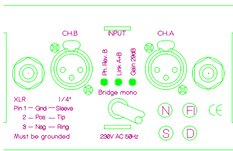
Figure 5. Rear panel connectors
